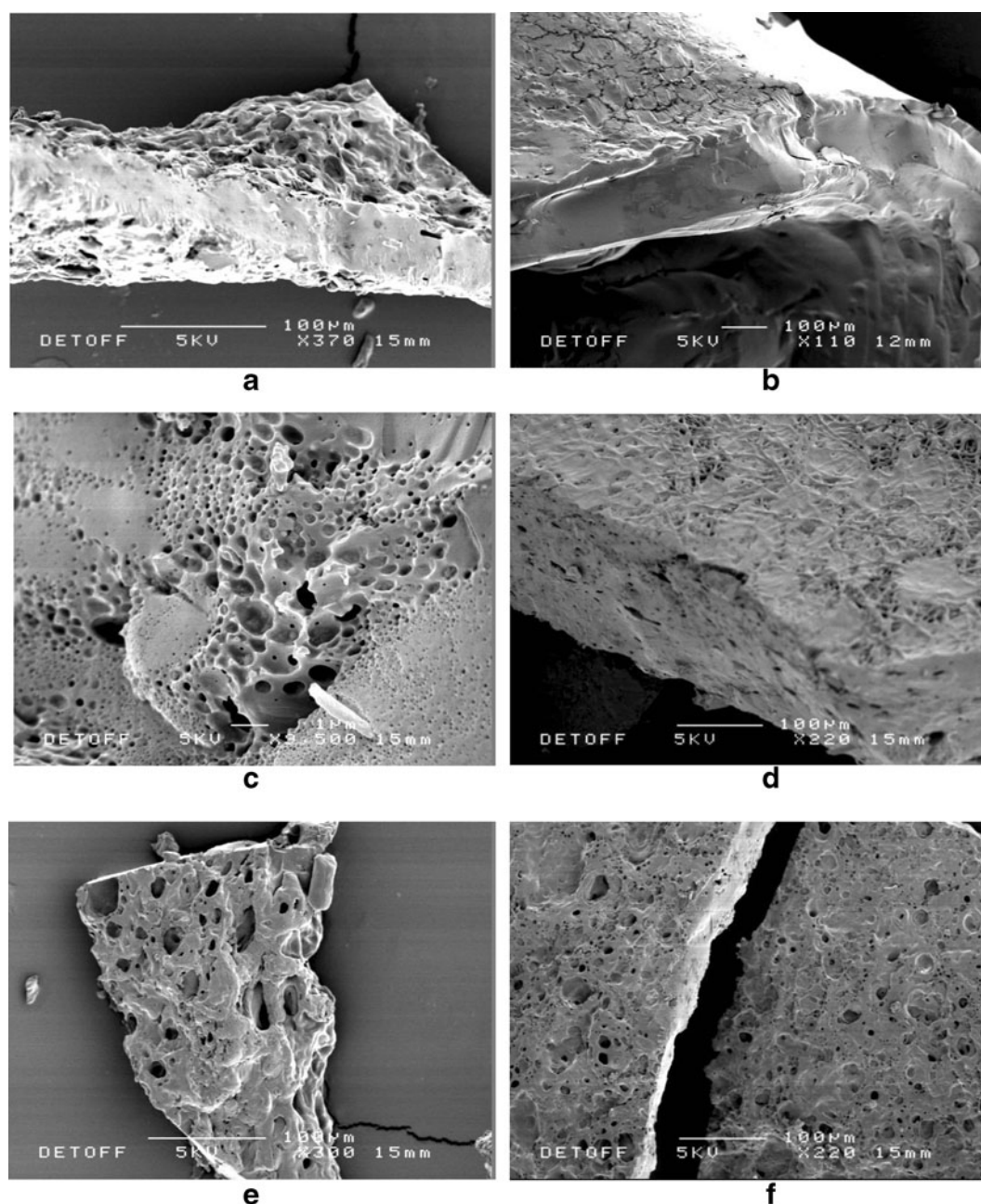
Fig. 4 SEM micrographs of degraded PLGA dressings loaded with amoxicillin and immersed in (a, b) distilled water, (c, d) PBS and (e, f) SBF after 25 days.
