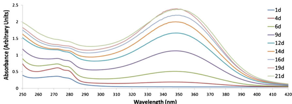
Fig. 8 Graph showing the concentration of the amoxicillin degradation product piperazine 2,5-dione, increasing over the period of 21 days.
