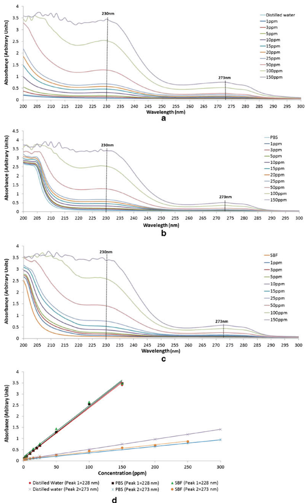
Fig. 6 UV spectra for different amoxicillin concentrations, when dissolved in (a) distilled water, (b) PBS and (c) SBF. The amoxicillin calibration curves for the 3 media are shown in graph (d). These curves were used in preparing the in vitro drug release profiles for the dressing patches and their R^2 values were > 0.99 .
