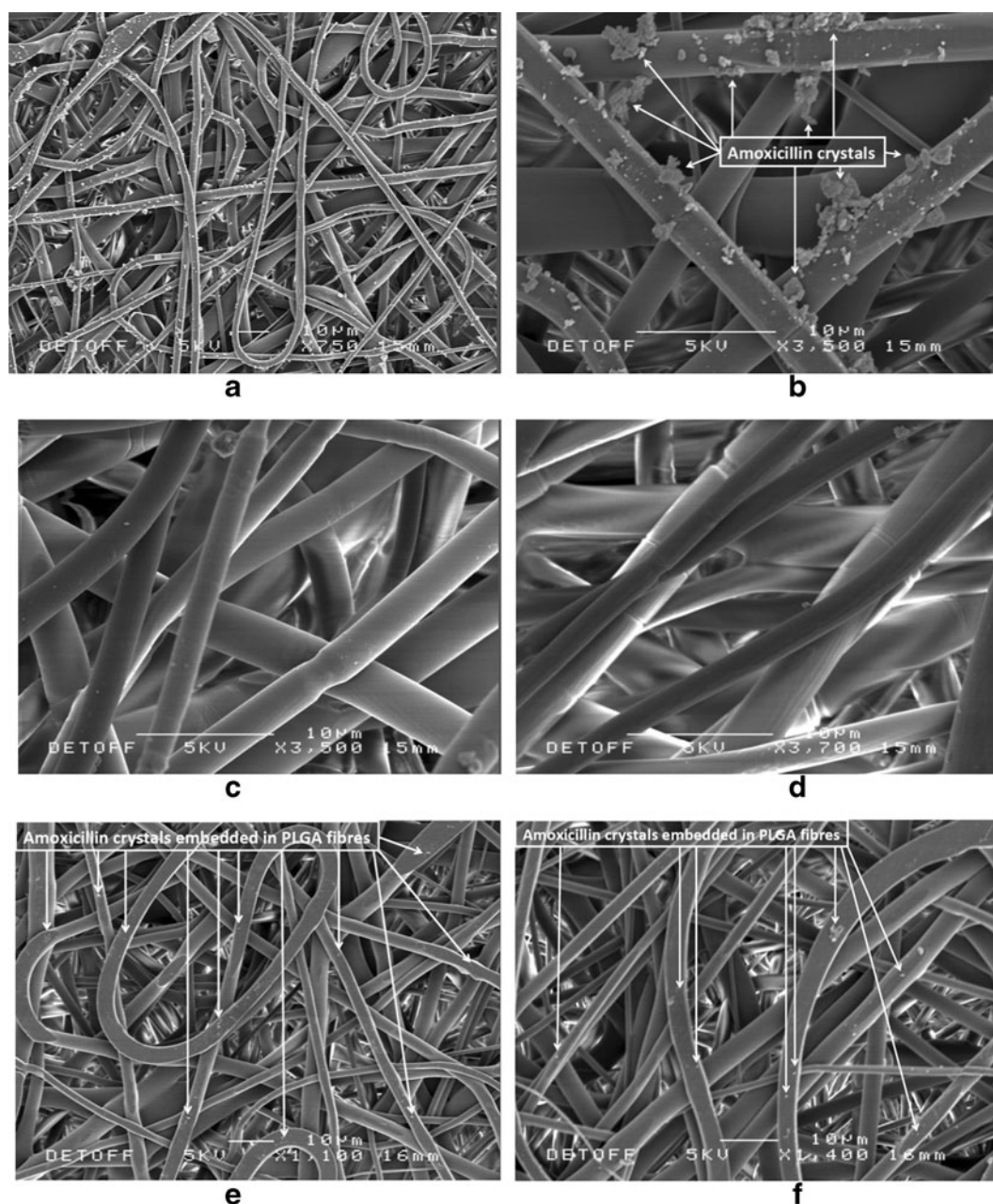
Fig. 2 SEM micrographs of electrospun PLGA microfibres ( a, b ) with and ( c, d ) without amoxicillin. The crystals attached to the fibre surfaces shown in ( b ) with arrows are amoxicillin. Micrographs ( e ) and ( f ) show sectioned PLGA fibres where the white areas shown with arrows indicate the amoxicillin embedded in them.
